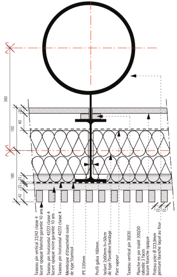
PLAN 1/10°
